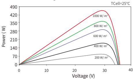
Power-Voltage Curves (48QL6-DV 475W)
