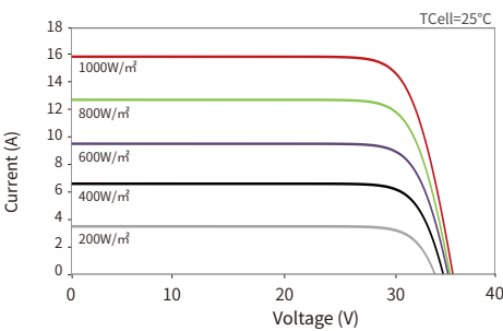
Current-Voltage Curves (48QL6-DV 475W)
